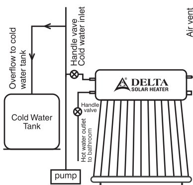
Manual water feeding system
