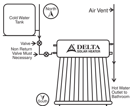
Overhead tank water feeding system
