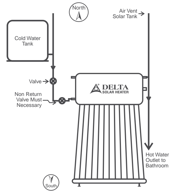
Over head tank water fitting system
